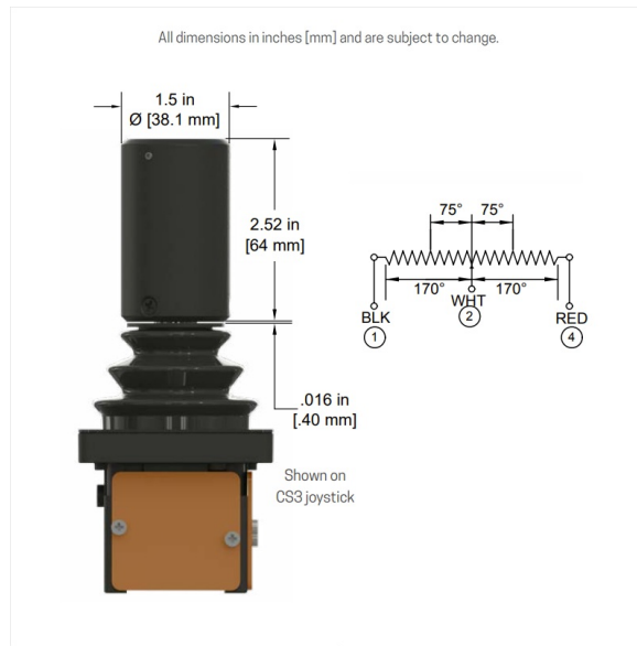
TH30 dimensions and wiring details
