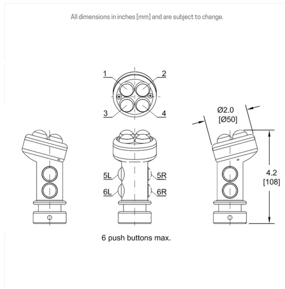
MG25 device locations & dimensions
