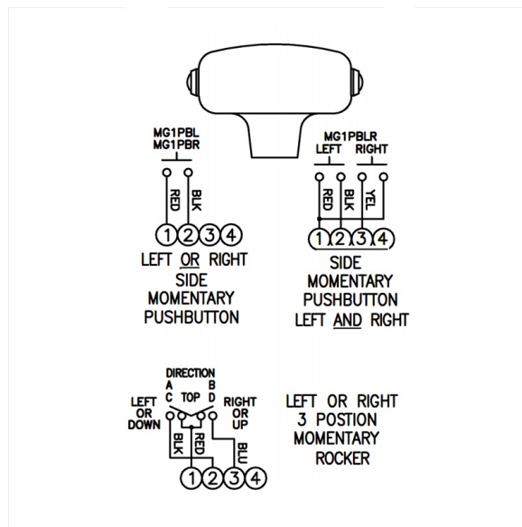
MG1 button and rocker switch wiring details
