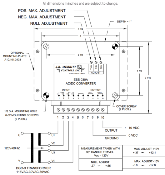
ESS 03A dimensions and wiring details
