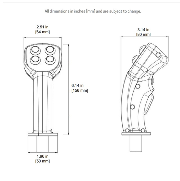
G58 dimensions
