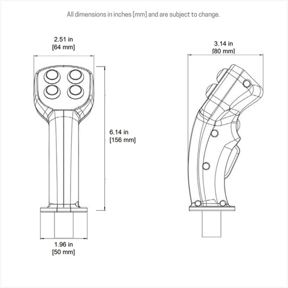
G58 dimensions
